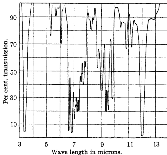
Fig. 8.—Infrared spectrum of p -diisopropylbenzene measured at 25^\circ , 0.051 mm. cell length.
