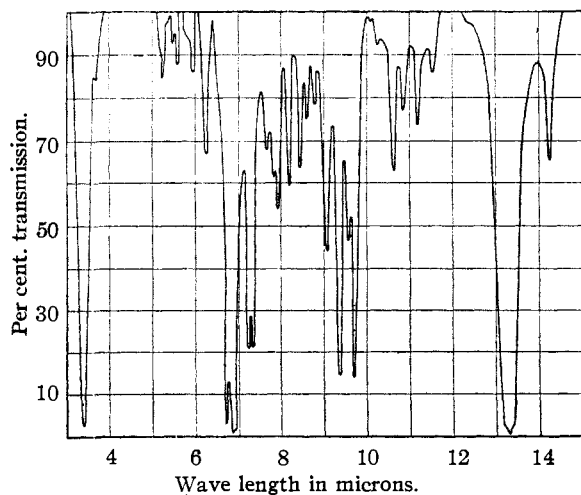
Fig. 6.—Infrared spectrum of o -diisopropylbenzene measured at 25^\circ , 0.051 mm. cell length.
