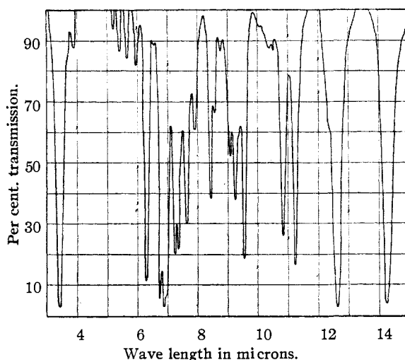
Fig. 7.—Infrared spectrum of m -diisopropylbenzene measured at 25^\circ , 0.051 mm. cell length.
